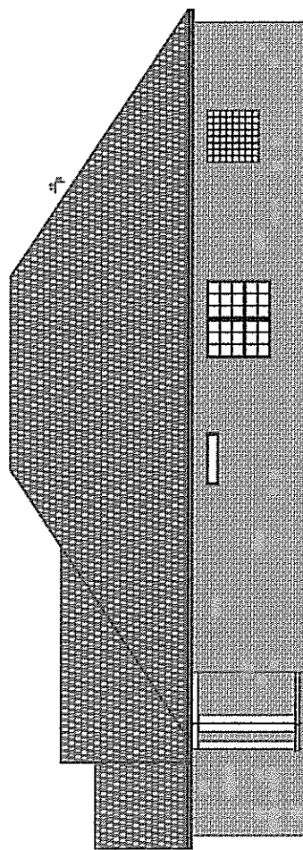
RIGHT SIDE ELEVATION SCALE 1/8" = 1'-0"
